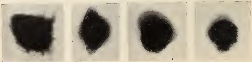
Strain 221.
